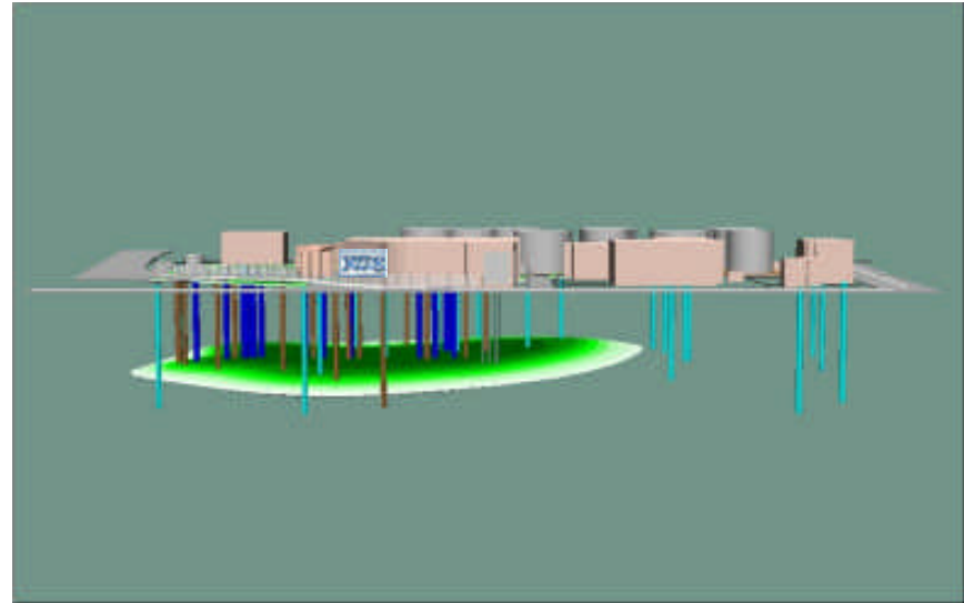
Free Product Plume Below ARCO and IWC Sites (Cross-section View)
